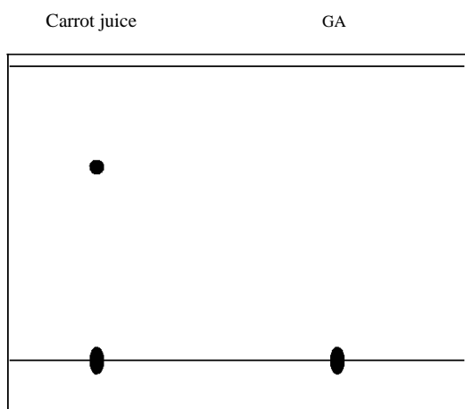
Figure 6. Sketch of the paper chromatogram of pure GA and carrot juice after staining with iodine (not to scale).
