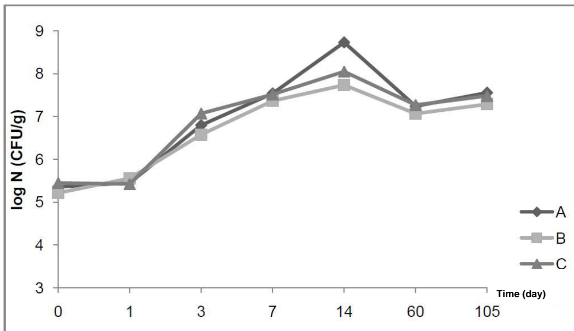
Figure 2. Total plate count growth dynamics during ripening and storage of Sremska sausage.
