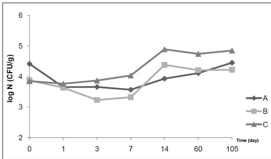
Figure 4. Gram positive and catalase positive cocci growth dynamics during ripening and storage of Sremska sausage.
