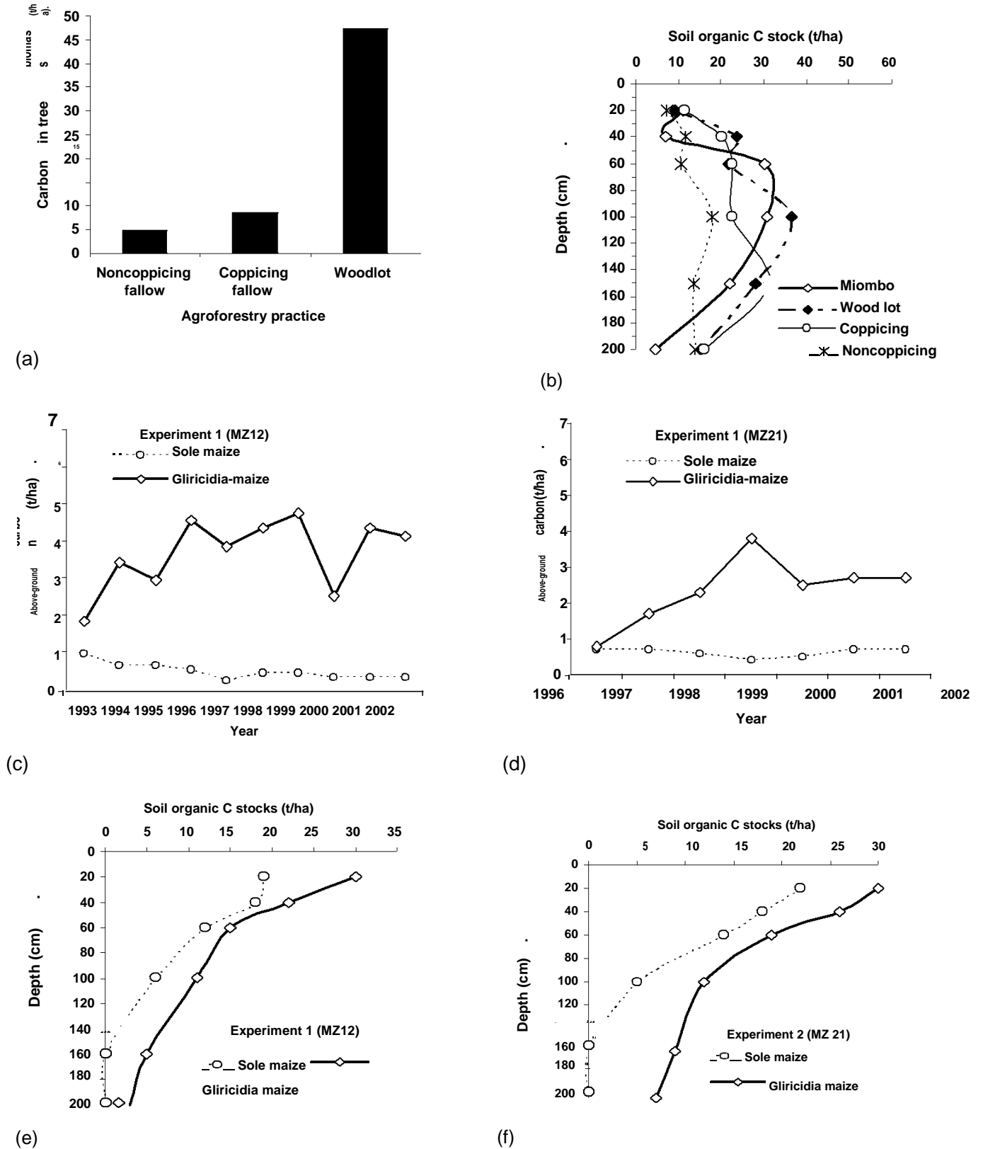
Figure 1. (a) Carbon storage in tree biomass and (b) stocks in the soil depths under woodlots, Miombo woodland, and coppicing and noncoppicing fallows at Msekera, Zambia (Source: Kaonga, 2003); (c & d) organic carbon recycled via the organic materials and (e & f) organic carbon in the soil profile in gliricidia-maize intercropping and sole maize in two experiments at Makoka, Malawi (Source: Makumba, 2003). Woodlots were 12 year old trees of Leucaena species; coppicing fallows were two to 7 year old Gliricidia , Leucaena spp., Senna , calliandra ; noncoppicing fallows were two-year-old Sesbania sesban , Tephrosia spp. and pigeon pea (Source: Kaonga, 2003).
