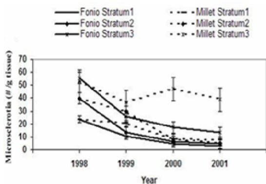
Figure 1. Evolution of microsclerotial soil inoculum density of Macrophomina phaseolina over 4 years in three plots with moderate (Stratum1), high (Stratum2), and very high (Stratum3) inoculum density after cropping cowpea in 1997 (before planting cereals in 1998), and after cropping the nonhosts fonio and millet in 1998, 1999, and 2000. Vertical lines indicate the standard error (to be improved).
