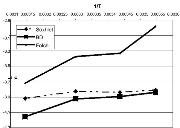
Figure 1. Arrhenius plot of Solanum nigrum L seed oil.
