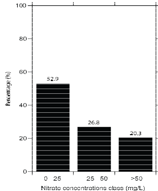
Figure 3. Frequency distribution of \text{NO}_3^- contents.
