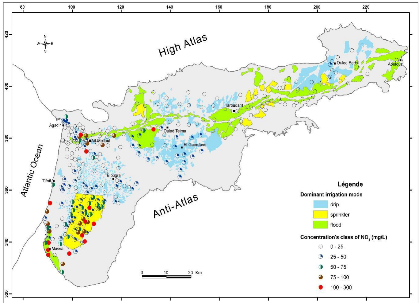
Figure 4. Spatial distribution of \text{NO}_3 contents overlaid to the irrigation type used in Souss-Massa region.
