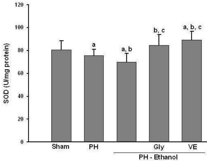
Figure 4. Effect of glycine and vitamin E on (SOD) activity in liver from all ethanol-treated groups during liver regeneration. Values are means \pm Standard error of mean (SE) (n = 10). SOD activity was expressed as U/mg protein. a P < 0.05 vs. the sham group (sham); b P < 0.05 vs. the hepatectomized group (PH); c P < 0.05 vs. hepatectomized + ethanol group (PH-EtOH). PH: Partial hepatectomy; Gly: Glycine; VE: Vitamin E.
