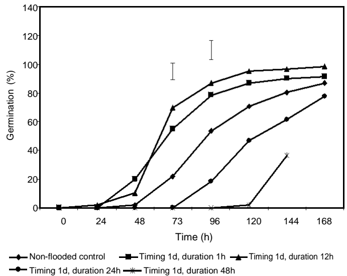
Figure 4. The effect of flooding at 1 day after start of imbibition on the time course of germination of bambara groundnut seeds. Vertical bars indicate standard error of the mean.
