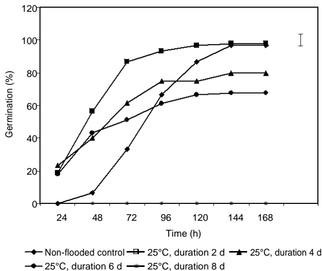
Figure 2. The effect of flooding duration at 25°C on the time course of germination of bambara groundnut seeds. Error bar represents the SE of the difference between two means (n = 24).
