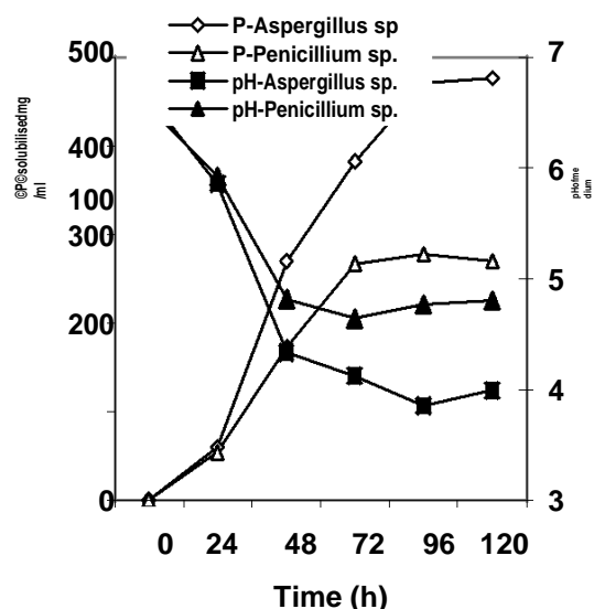
Figure 2. Kinetics of 'P' solubilization from tricalcium phosphate by Aspergillus sp. and Penicillium sp. in PVK medium.
