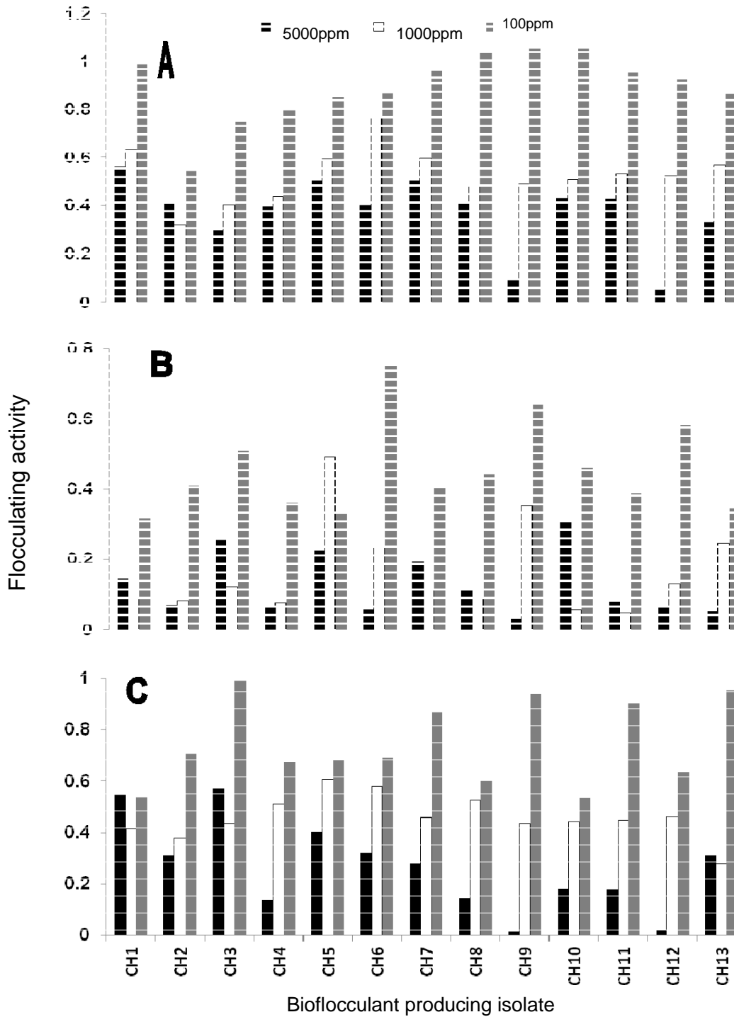
Figure 2. The effect of biofloculants concentrations on the flocculation activity in the presence of different metal (a) Pb^{2+} ; (b) Zn^{2+} and (c) Hg^{2+} .
