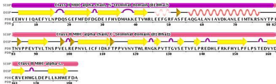
Figure 3. Molecular structure of Class II Histocompatibility antigen (HLA-DR1) (PDB ID: 1DLH) revealing binding domain in beta sheets representation of secondary structure sequence.
