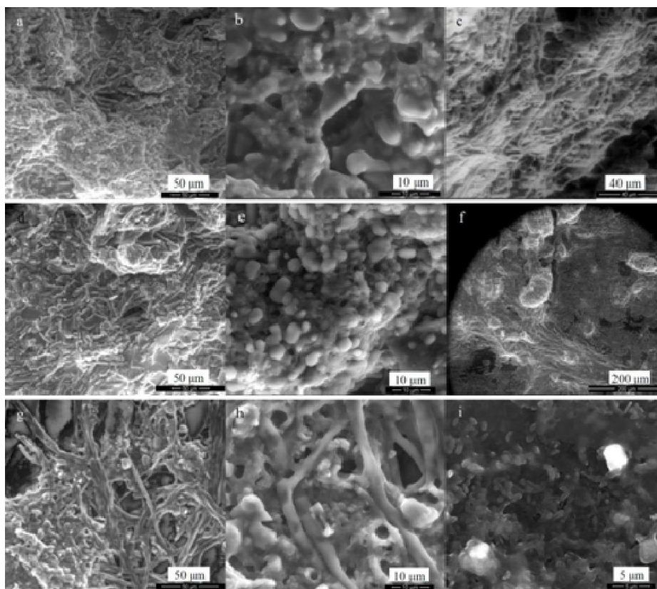
Figure 2. ESEM images of suspended carrier biofilm from M1 (a, b, c), M2 (d, e, f) and M3 (g, h, i).
