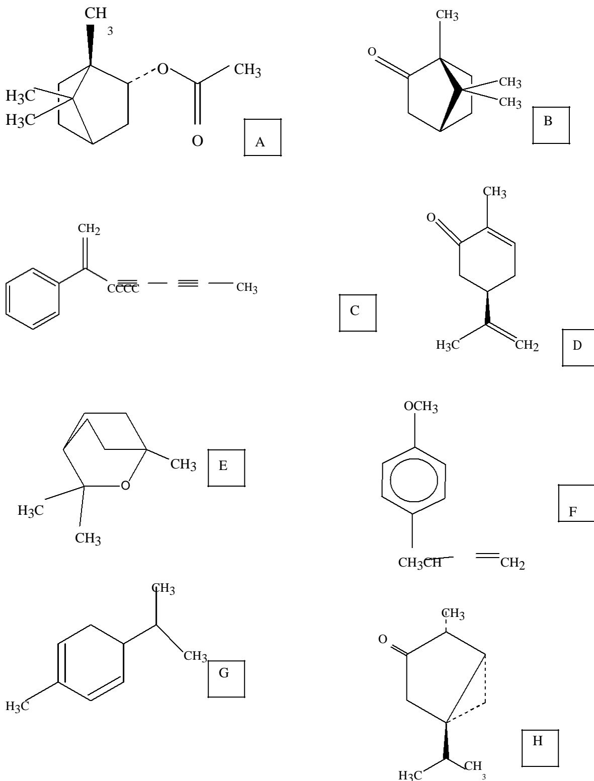
Figure 1. Chemical structure of some principle (> 40% of oil, relative %) compounds in Anthemideae species essential oils. A) bornyl acetate, B) (D) camphor, C) capillene, D) R-(-)-carvone, E) 1,8-cineole, F) estragol, G) \alpha -phellandrene, H) \beta -thujone.
