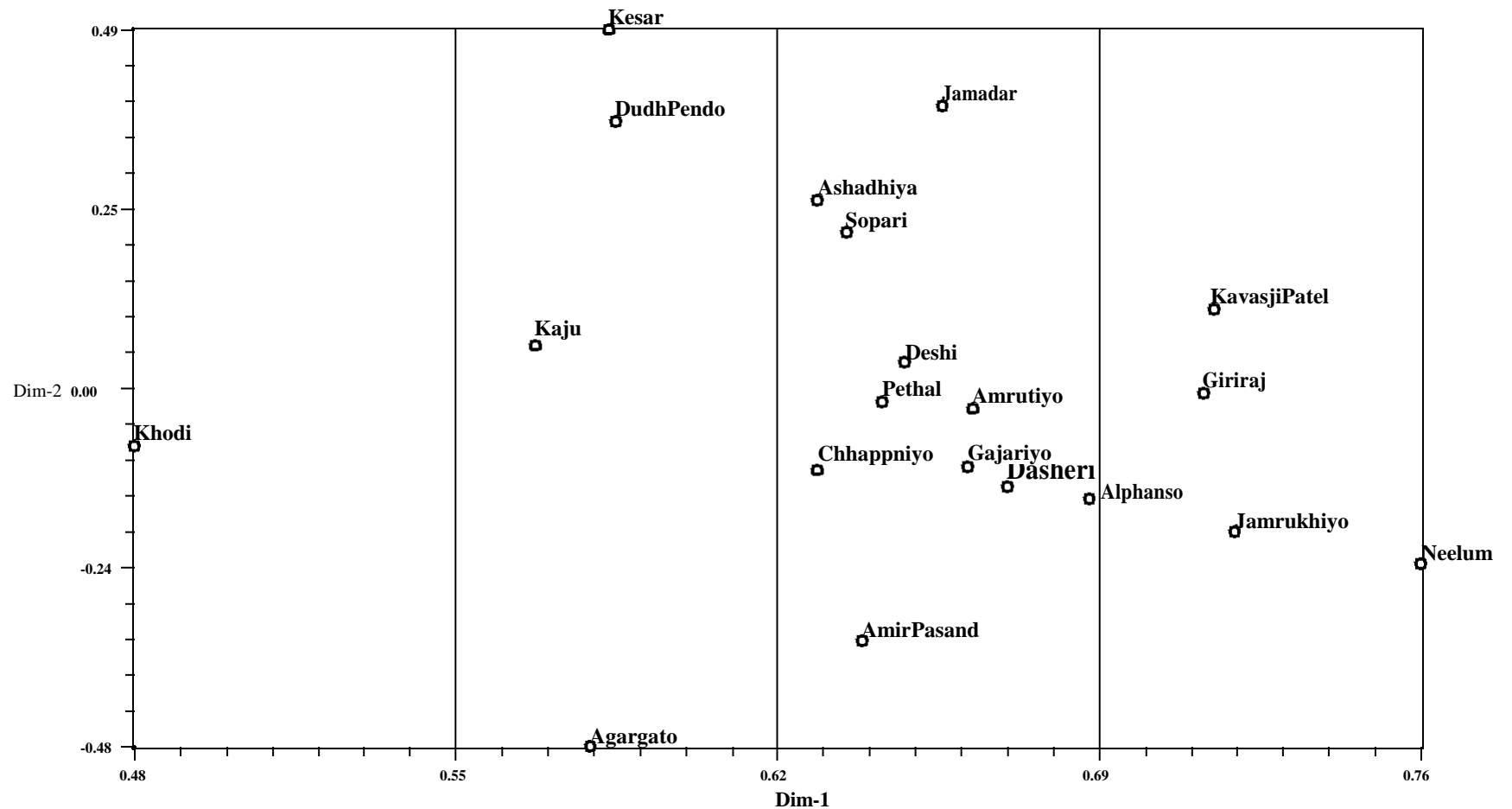
Figure 2. Principal coordinate analysis of 20 mango landraces using ISSR markers.
