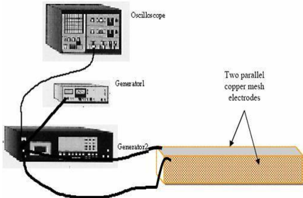
Figure 1. The electromagnetic field treatment system.
