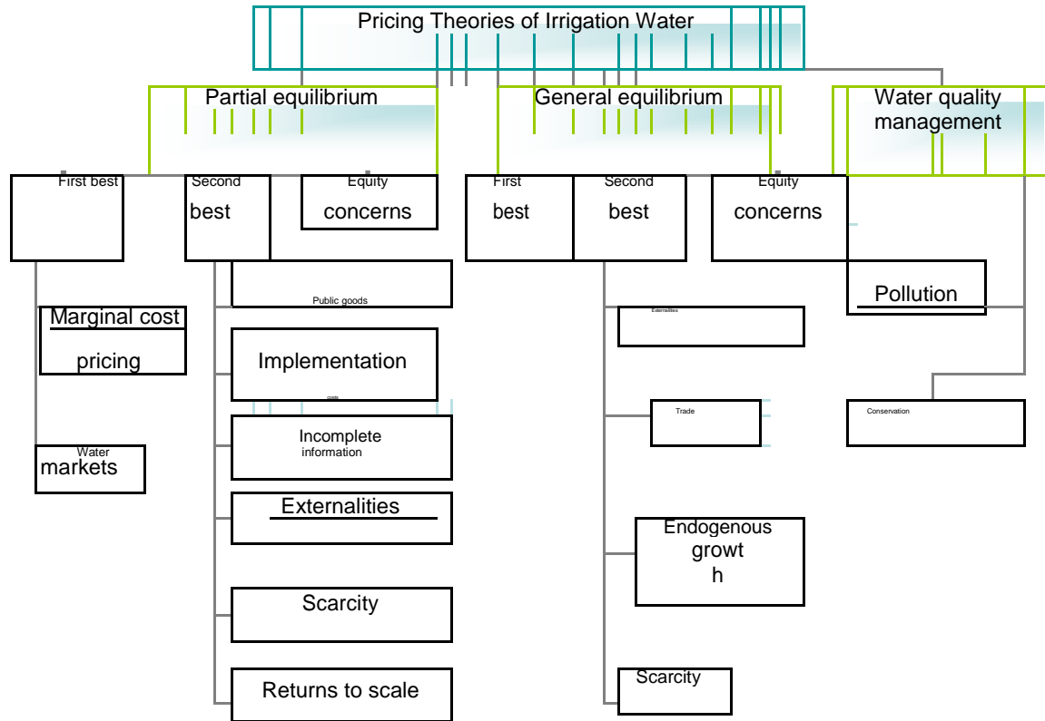
Figure 1. Schematic of normative theories of irrigation water pricing.
