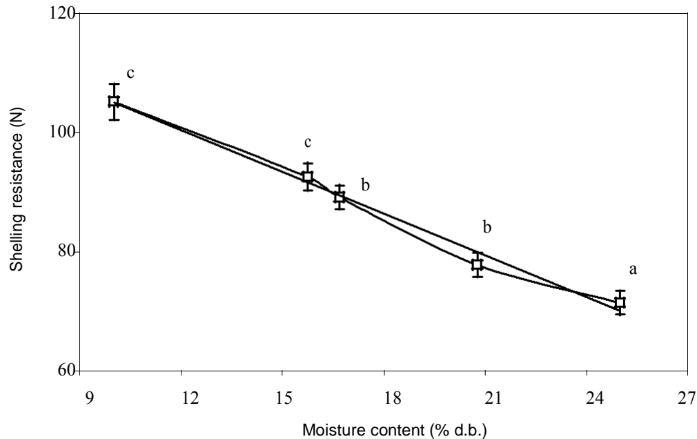
Figure 10. Effect of moisture content on shelling resistance of white kidney beans. a-c Values followed by different letters are significant at P<0.05.
