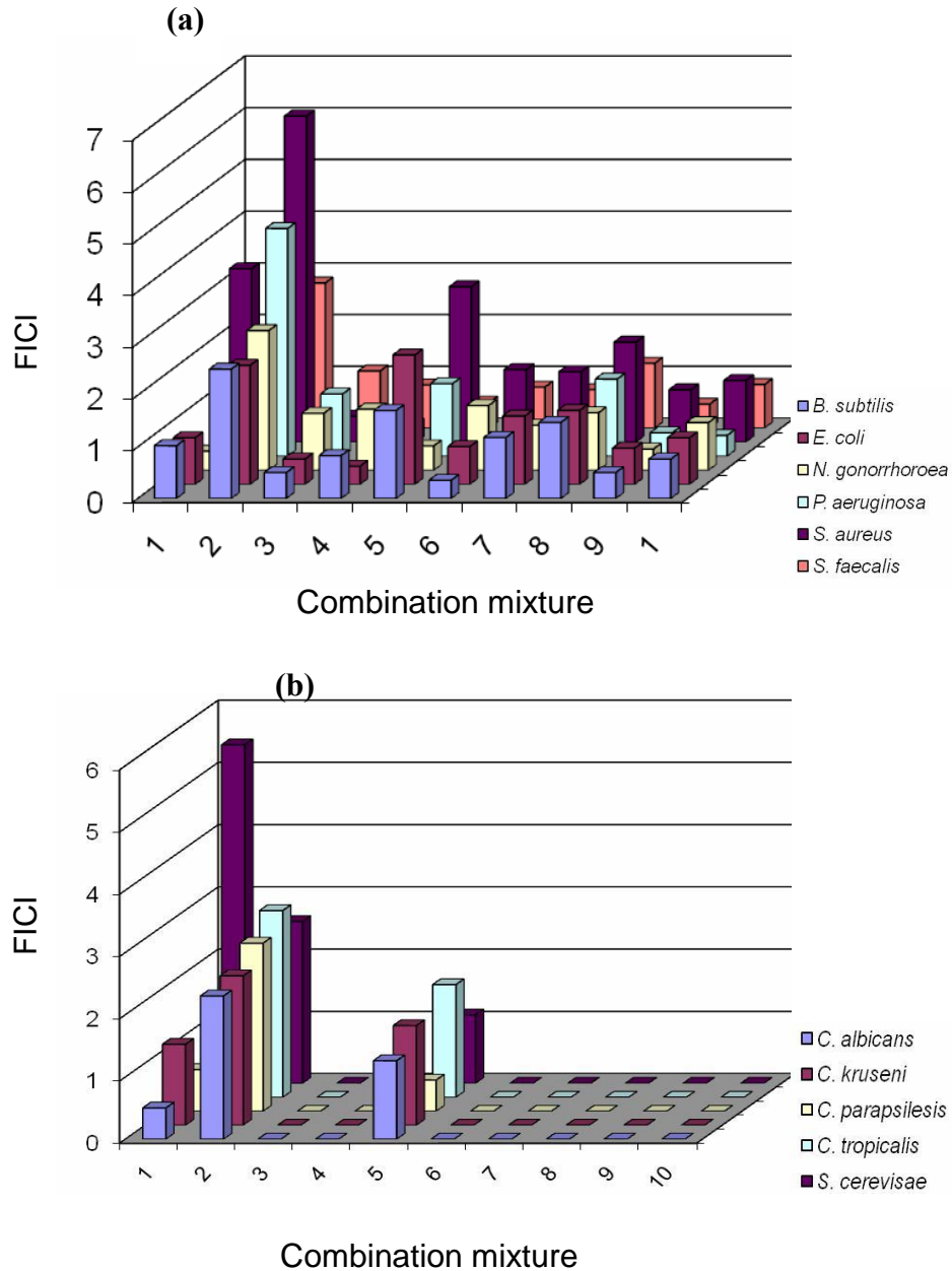
Figure 3. Combination antimicrobial of dual active constituents separated from of M. peregrina (Bacteria (P < 0.03, F = 2.1), Fungi (P < 0.03, F = 1.9)). Combination mixtures: 1: Lupeol acetate + \beta -amyryn, 2: Lupeol acetate + \alpha -amyryn, 3: Lupeol acetate + \beta -sitosterol, 4: Lupeol acetate + \beta -sitosterol-3-O-glucoside, 5: \beta -amyryn + \alpha - amyryn, 6: \beta -amyryn + \beta -sitosterol, 7: \beta -amyryn + \beta -sitosterol-3-O-glucoside, 8: \alpha -amyryn + \beta -sitosterol, 9: \alpha -amyryn + \beta -sitosterol-3-O-glucoside, 10: \beta -sitosterol + \beta -sitosterol-3-O-glucoside
