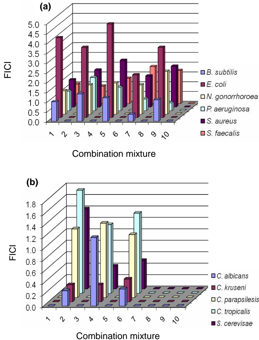
Figure 5. Combination antimicrobial therapy between active constituents separated from M. peregrina plus reference antibiotics from local market (Bacteria ( P < 0.01 , F = 1.9 ), Fungi ( P < 0.02 , F = 0.9 )). Combination mixtures: 1: Lupeol acetate + ampicillin, 2: Lupeol acetate + fluconazole, 3: \alpha -amyrin + ampicillin, 4: \alpha -amyrin + fluconazole, 5: \beta -amyrin + ampicillin, 6: \beta -amyrin + fluconazole, 7: \beta -sitosterol-3-O-B-d glucoside + ampicillin, 8: \beta -sitosterol + fluconazole, 9: \beta -sitosterol + ampicillin, 10: \beta -sitosterol-3-O-glucoside + fluconazole
