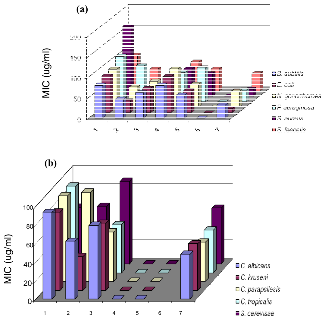
Figure 2. MIC for the active constituents separated from Moringa Peregrina for (a) Bacteria ( P < 0.02 , F = 2.1 ) and (b) Fungi ( P < 0.03 , F = 1.2 ). 1: Lupeol acetate, 2: \beta -amyirin, 3: \alpha -amyirin, 4: \beta -sitosterol, 5: \beta -sitosterol-3-O-glucoside, 6: apigenin, 7: ampicillin or fluconazole (standard drugs).
