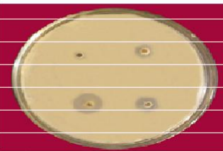
Antibacterial activity of [CoCl (TBHTSC) (Gly)]H 2 O against E. coli
