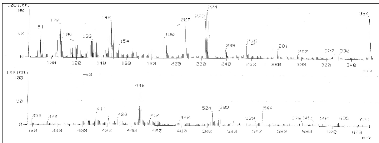
Figure 3. (a) Splitting patterns of FAB mass of [intensity vs m/z](a) [\text{CoCl}(\text{C}_{11}\text{H}_{17}\text{N}_3\text{S})(\text{C}_2\text{H}_5\text{NO}_2)]\text{H}_2\text{O}
