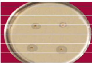
Antibacterial activity of TBHTSC against E. coli
