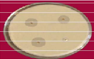
Antibacterial activity of TBHSC against E. coli
