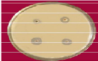
Antibacterial activity of TBHSC against S. aureus
