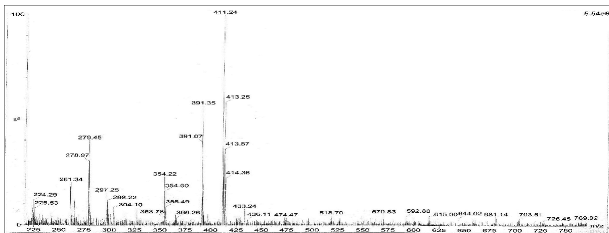
Figure 3. (b) [\text{CuCl}(\text{C}_{11}\text{H}_{17}\text{N}_3\text{S})(\text{C}_2\text{H}_5\text{NO}_2)]\text{H}_2\text{O}
