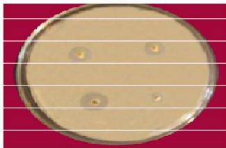
Antibacterial activity of [CoCl (TBHTSC) (Gly)]H 2 O against S. aureus
