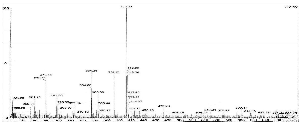
Figure 3. (c) [\text{CuCl}(\text{C}_{11}\text{H}_{17}\text{N}_3\text{S})(\text{C}_3\text{H}_7\text{NO}_2)]\text{H}_2\text{O}
