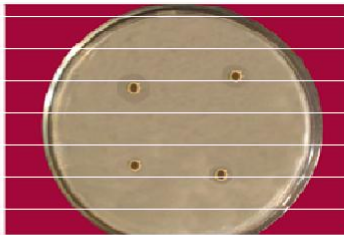
Antifungal activity of IPMCHTSC against C. albicans
