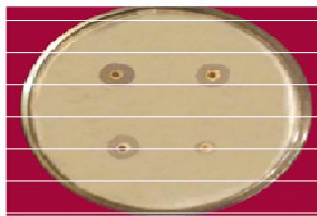
Antibacterial activity of IPMCHTSC against E. coli
