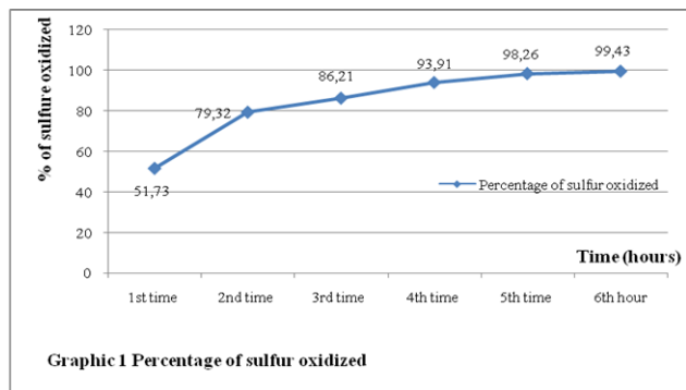
Graphic1. Sulfur oxides as a function of time
